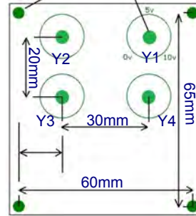
SWITCHBOARD FRONT VIEW
