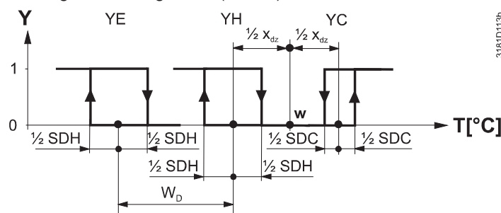
Heating and cooling mode (P01=4)
