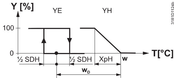
Heating mode with manual selection (P01=2)
