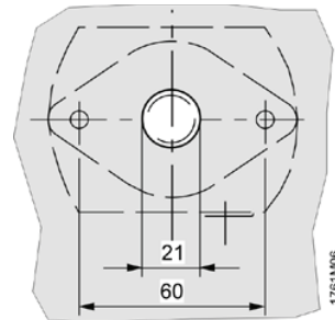
Drilling plan
